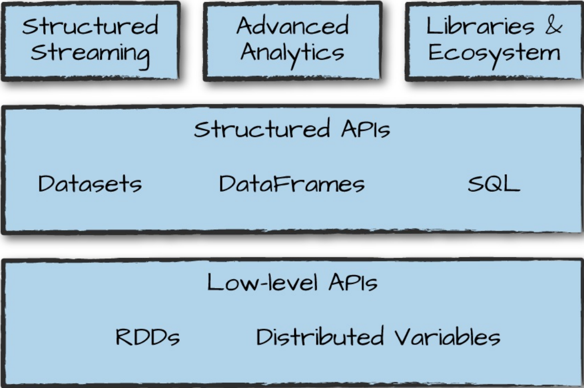
Figure 3-1. Spark's toolset
